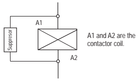
Wiring diagram of suppressor in contactors
