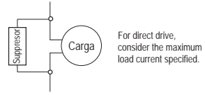
Wiring diagram of suppressor linking in loads direct drive
